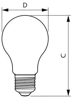
A70 230V 11-100W 1521lm 2700K E27 ND
